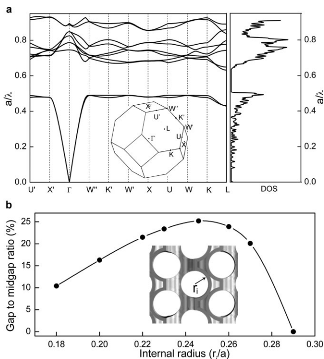
Figure 1. a) Band structure and density of states of an inverse woodpile structure consisting of hollow Ge ( n=4.1 ) tubes with an internal radius of 0.25 a and an external radius of 0.306 a . The inset shows the Brillouin zone and its most important symmetry points. b) Dependence of the gap to midgap ratio as a function of the internal radius of these hollow tubes. The inset shows a (100) facet where the internal radius of the hollow rods is depicted.
