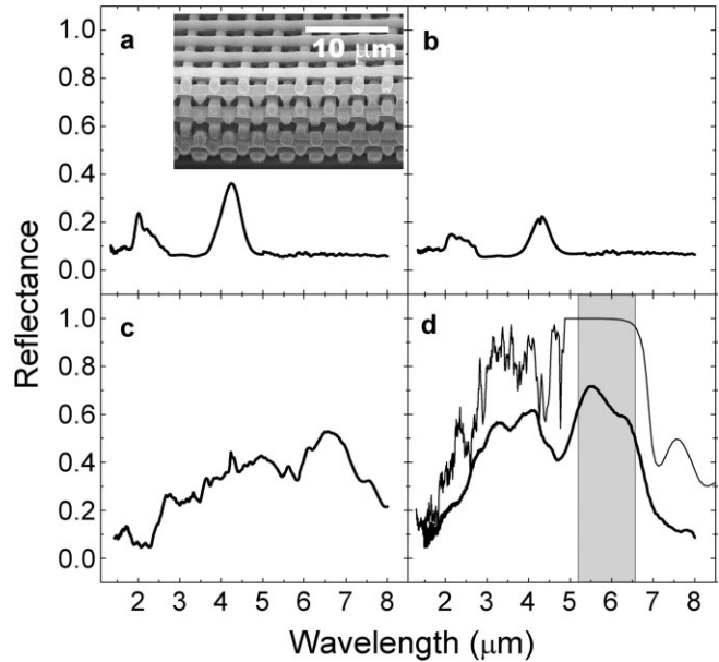
Figure 4. Reflectance spectra at different stages of fabrication. a) Initial polymer woodpile structure (inset shows an SEM cross section); b) oxide-coated polymer woodpile structure; c) Ge/oxide-coated, polymer woodpile structure; d) experimental (thick line) and simulated (thin line) Ge inverse woodpile structure. The lightly shaded region depicts the PBG.
