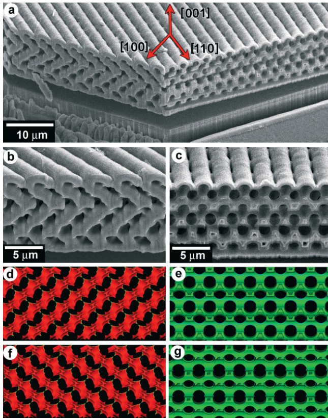
Figure 3. Inverse Ge woodpile structure. a) SEM image showing the surface of the sample with two edges exposed by FIB milling, with their orientations indicated. b,c) SEM higher resolution images of exposed (100) and (110) planes, respectively. Both images are taken with the substrate tilted 55°. d,e) Computer-rendered images of the edges shown in (b) and (c), equivalently tilted at 55°. f,g) Cross-sectional cuts at slightly different positions also parallel to the (100) and (110) planes, respectively.
