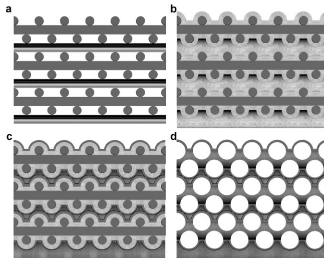
Figure 2. Fabrication scheme. a) Initial polymeric woodpile structure created by direct ink writing; b) thick film of an oxide bilayer conformally grown around the polymeric rods via ALD and CVD; c) infilling of the remaining pore volume with Ge via CVD; d) removal of the oxide and polymeric materials to yield a Ge inverse woodpile structure.
